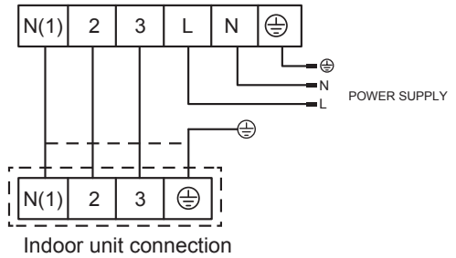
Outdoor Unit
